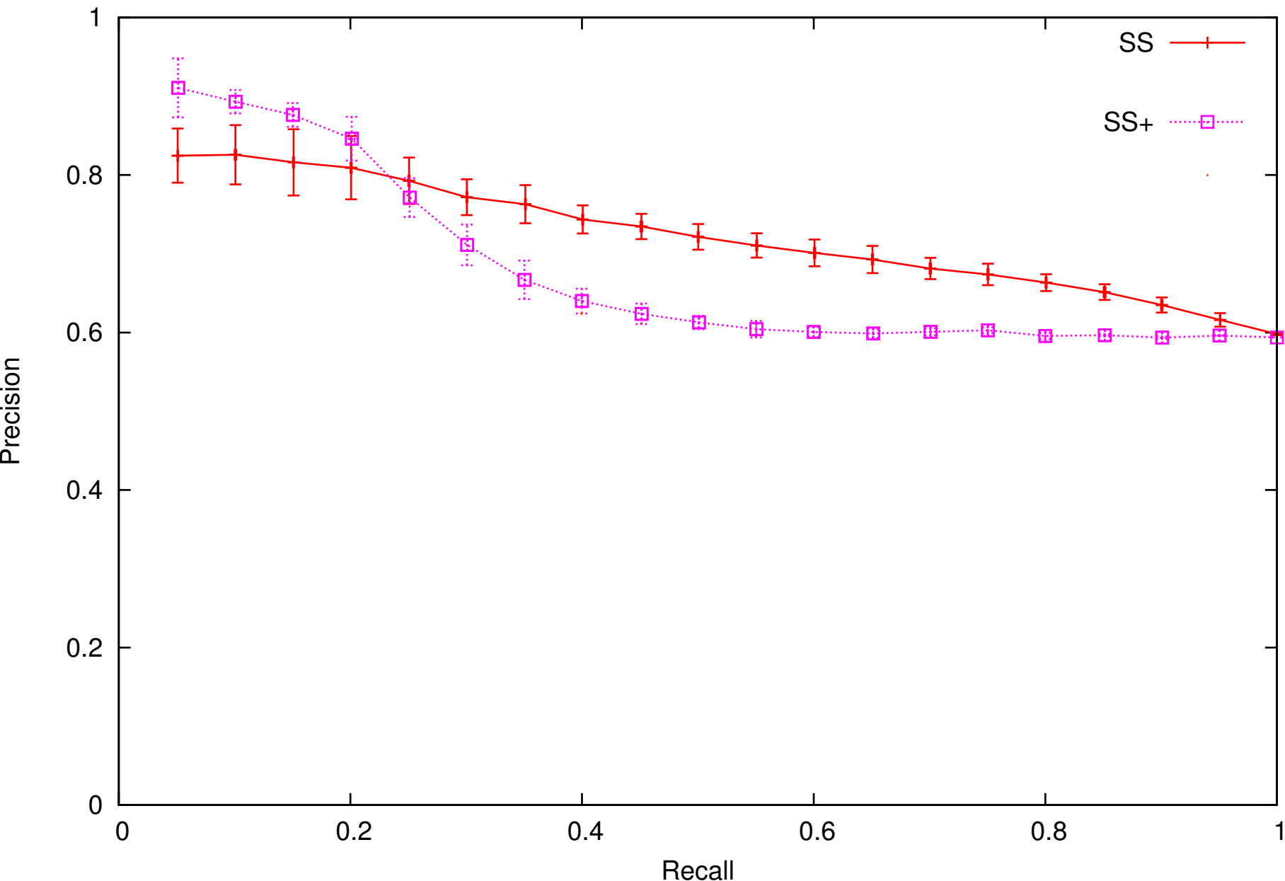
Brass-Konig-Zhou HDFs, unweighted network
