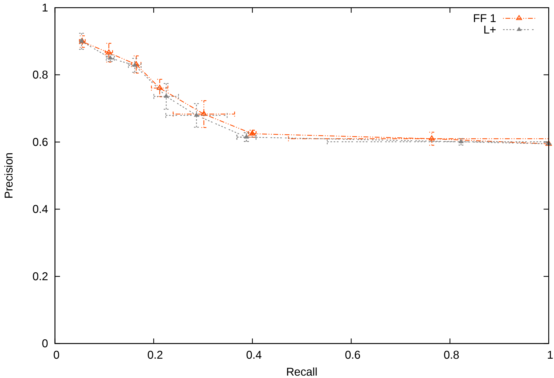
Brass-Konig-Zhou HDFs, unweighted network
