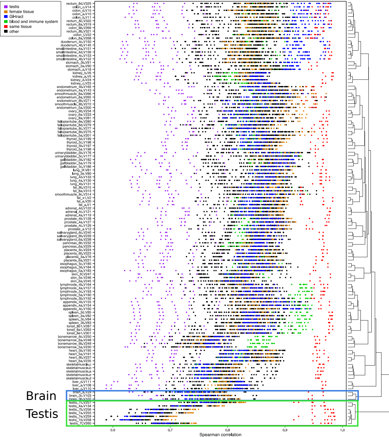
Pair-wise correlations within RNA-seq samples
