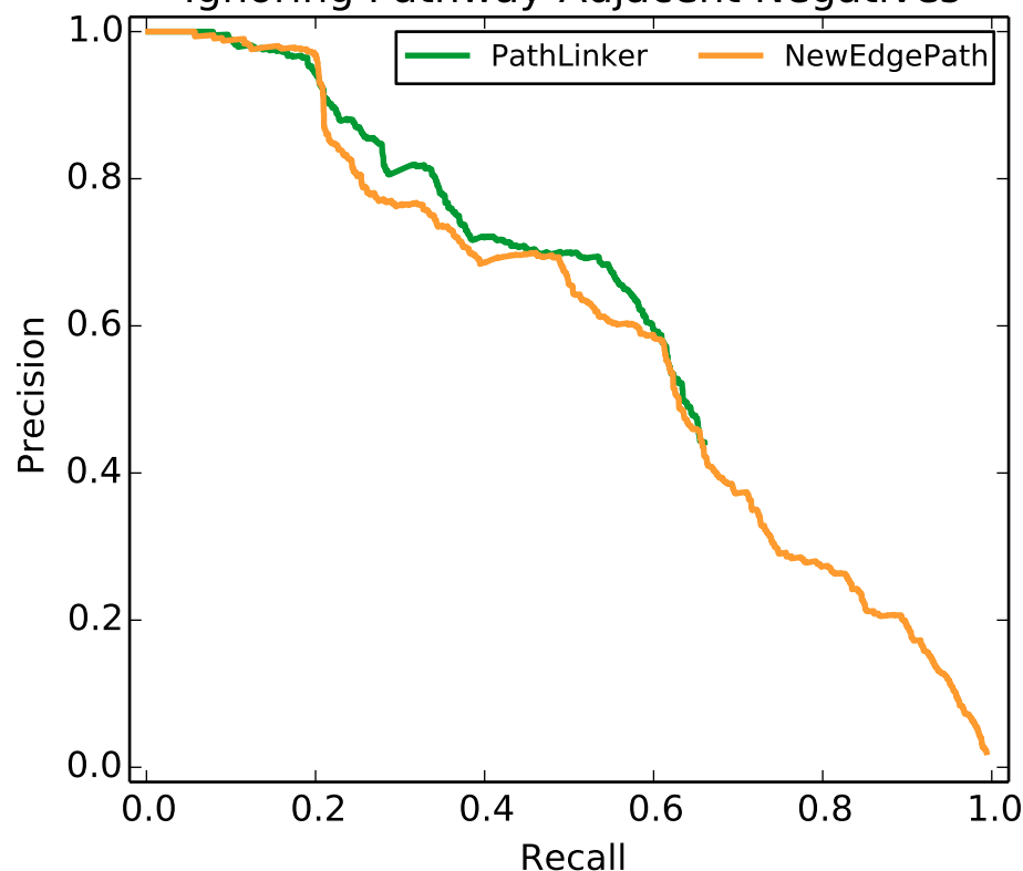
Interactions Aggregated over 15 Reconstructions Ignoring Pathway-Adjacent Negatives
