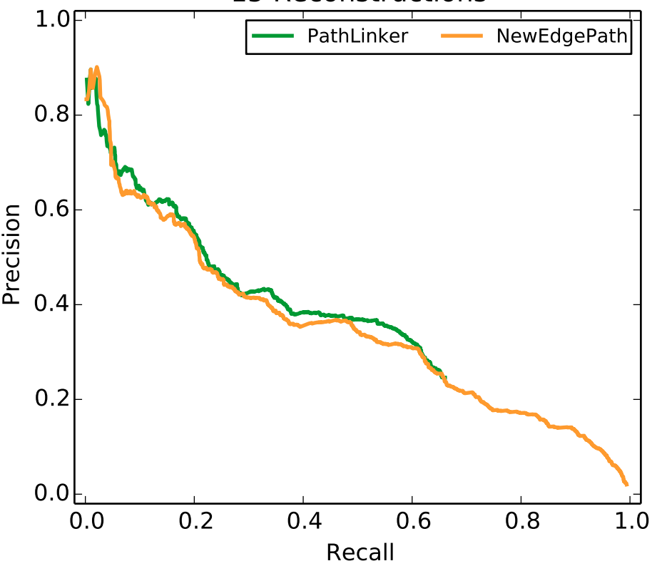
Interactions Aggregated over 15 Reconstructions
