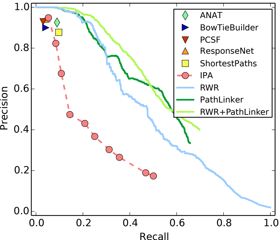
(a) Reconstructions of 29 NetPath Pathways
