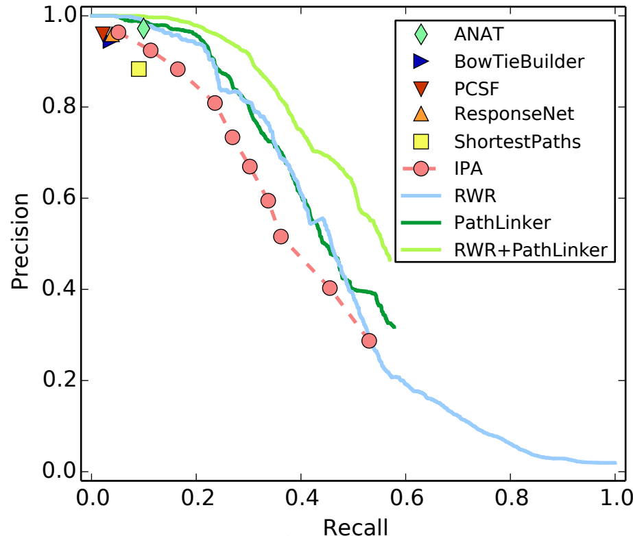
(b) Reconstructions of 32 KEGG Pathways
